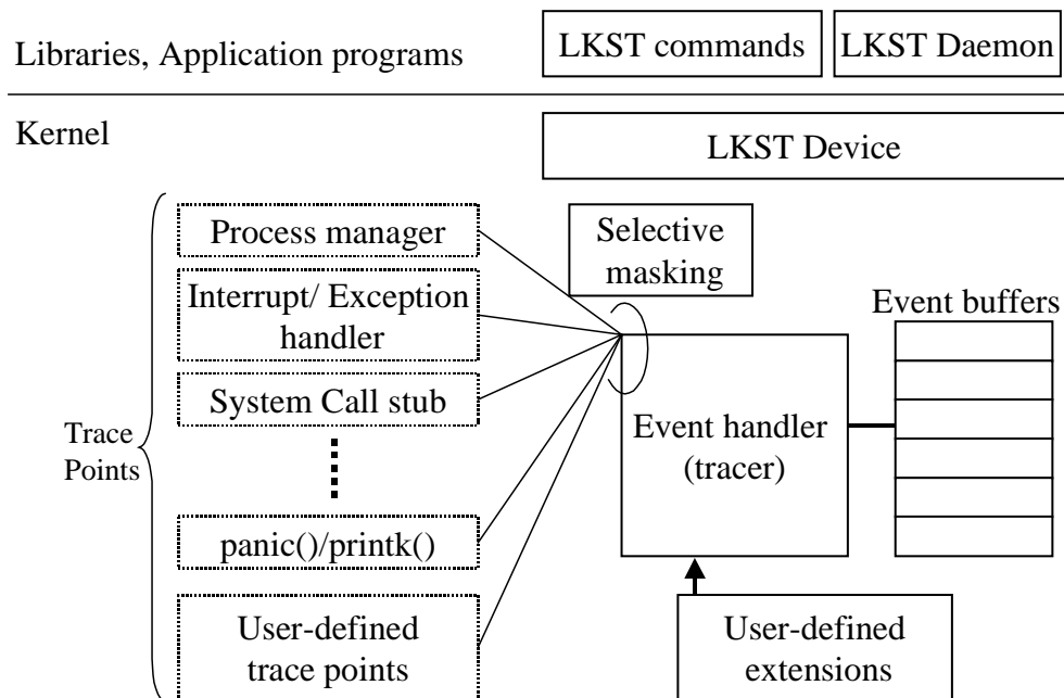
Figure 3-1. LKST block diagram.
