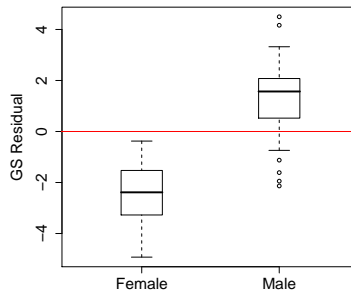
Figure 5: Boxplot of GS residuals for the Y-chromosome, obtained from a linear model with only phenotype as predictor and grouped by sex.
