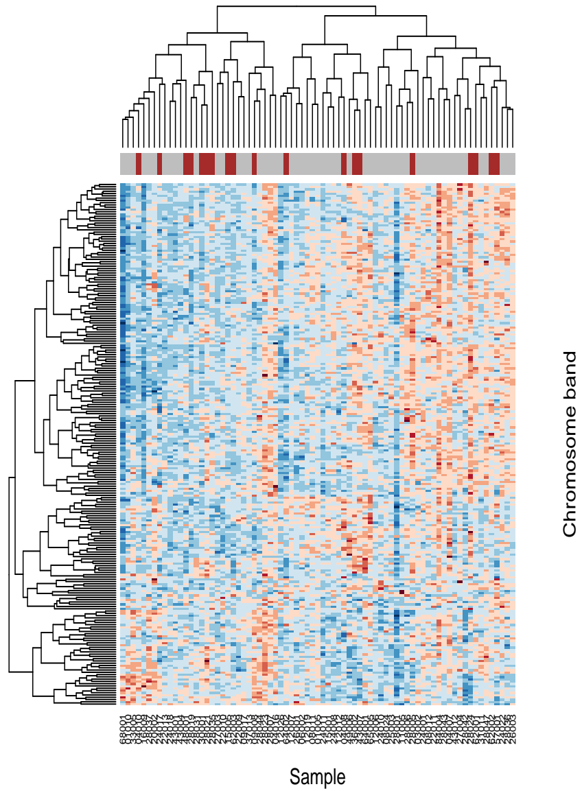
Figure 7: GS residuals from the 3-factor linear model. Layout and details are similar to those of Fig. 3.
