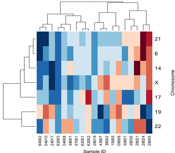
Figure 8: Complete-chromosome GS residuals from the 3-factor linear model, for chromosomes flagged as over-expressed under hyperdiploidy ( p < 0.1 ), and for the hyperdiploid subjects only.
