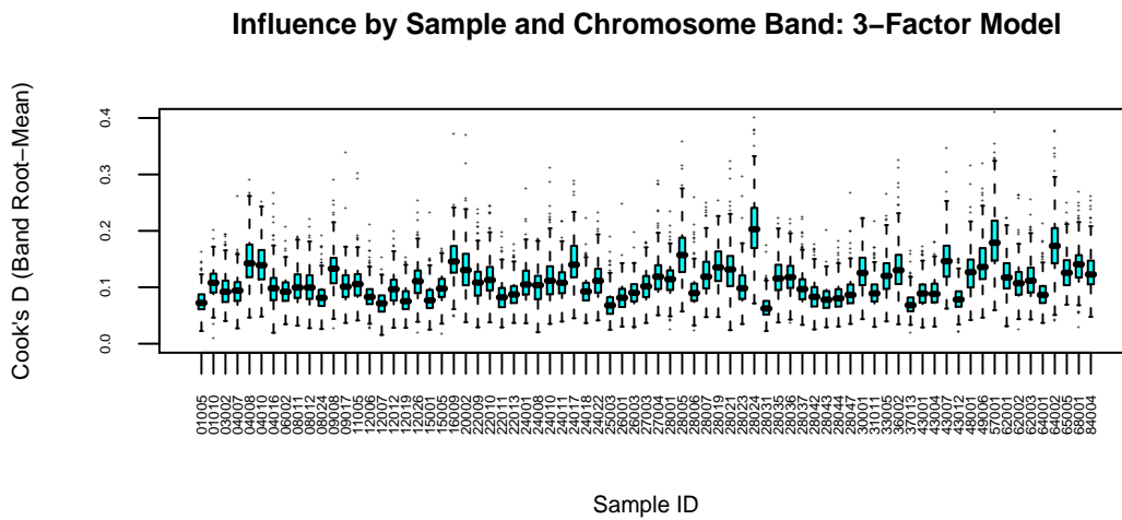
Figure 9: Chromosome-band root-mean Cook's D values, summarized by sample, for the 1-factor (top) and 3-factor (bottom) models.
